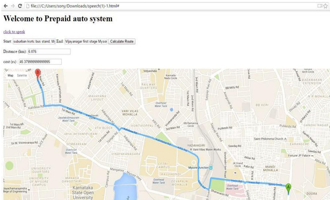
(a) Screen shot of speech recognition and distance module for Vijayanagar first stage, Mysuru, Karnataka, India
