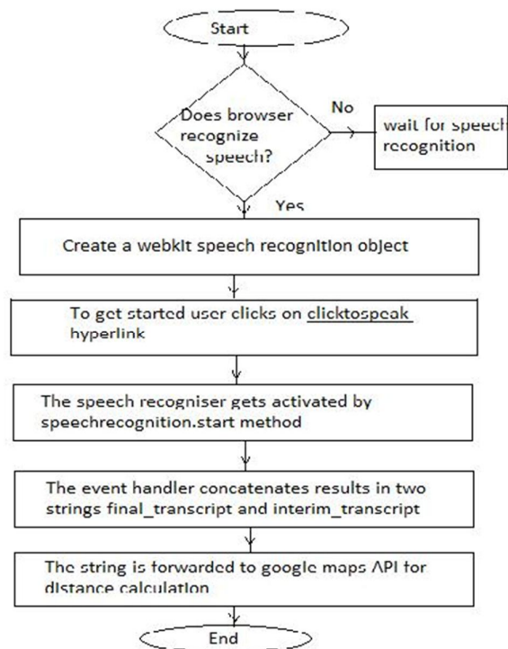
Figure 2: Flow of speech recognition
